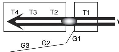
Figure 26.1. Schematic sketch of a directional freezing apparatus. Blocks can be set at different temperatures ( T_1 – T_4 ), thereby imposing a temperature gradient along the blocks ( G_1 – G_3 ).
